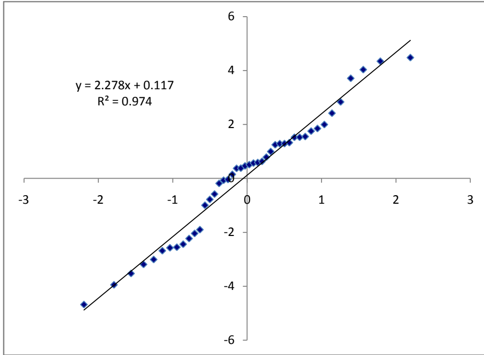
Figure 2. Normal Q-Q Chart of \ln(p_j/e_j) for Programming Time
