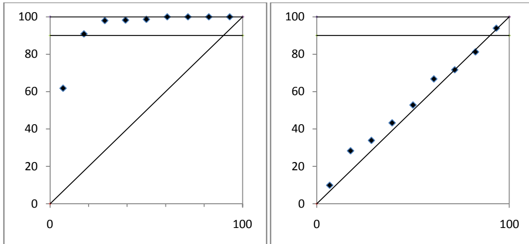
Figure 7. Nine Projects Results by PERT vs. Linear Association
