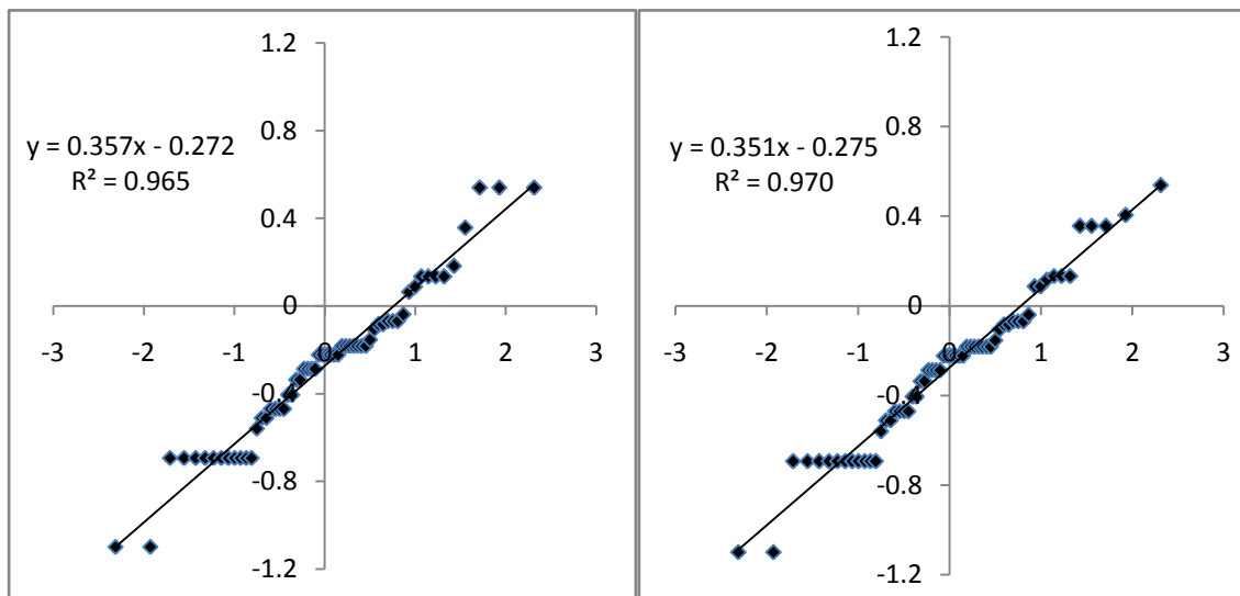
Figure 4. Q-Q Charts of \ln(p_j/e_j) for Two Trimmed Samples
