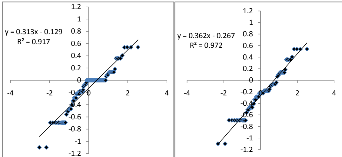
Figure 3. Q-Q Chart of \ln(p_j/e_j) in a Construction Project Showing the Parkinson Effect (left) and the Fit of the Parkinson Distribution (right)
