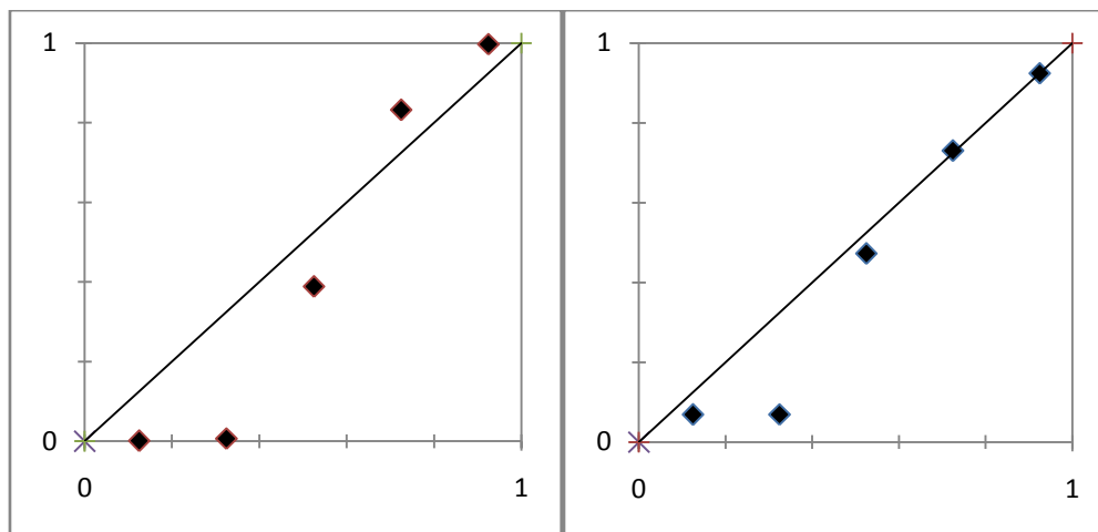
Figure 6. Five Projects: Calibrated Results vs. Linear Association
