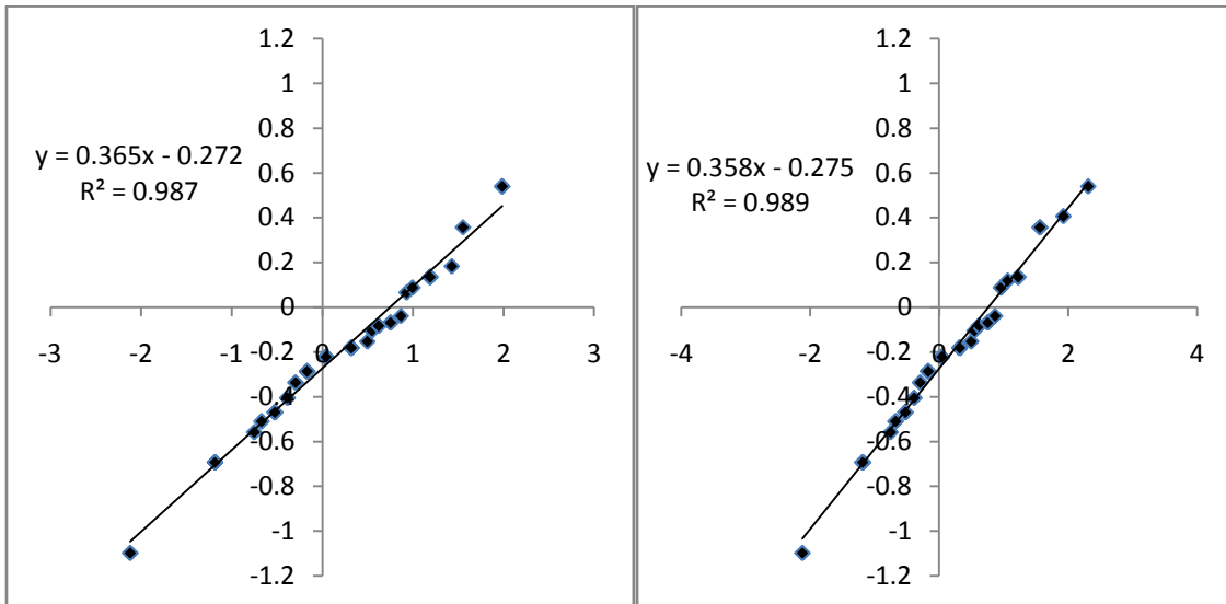
Figure 5. Resolving Ties by Using Average z -scores
